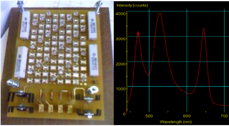
Prototype LED illumination system and an illustrated spectral power distribution.
