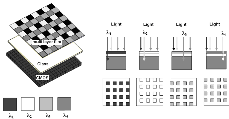
Figure 1 Four element color filter array
